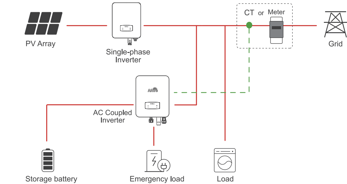
Single Phase AC Coupled (Retro Fit)
